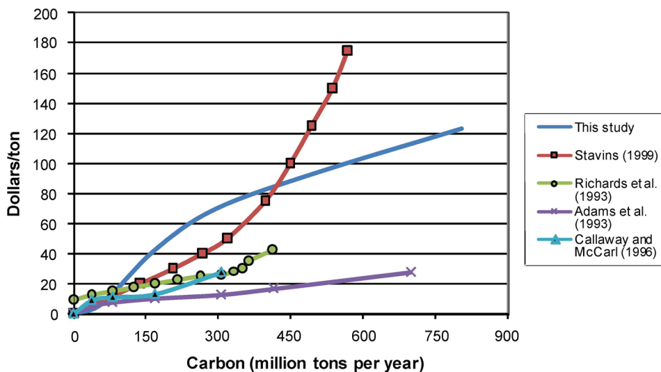
FIGURE 3.4 Comparison of marginal cost curves for forest carbon sequestration in the United States by Lubowski et al., 2006 with optimization models (Adams et al., 1993; Callaway and McCarl, 1996) and bottom-up engineering cost methods (Richards et al., 1993).
