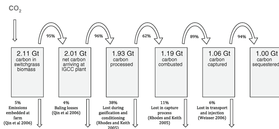
FIGURE 4.8 Carbon flows for switchgrass burned in an integrated gasification combined cycle facility retrofitted to burn biomass with carbon capture and sequestration. SOURCE: Smith and Torn, 2013.
