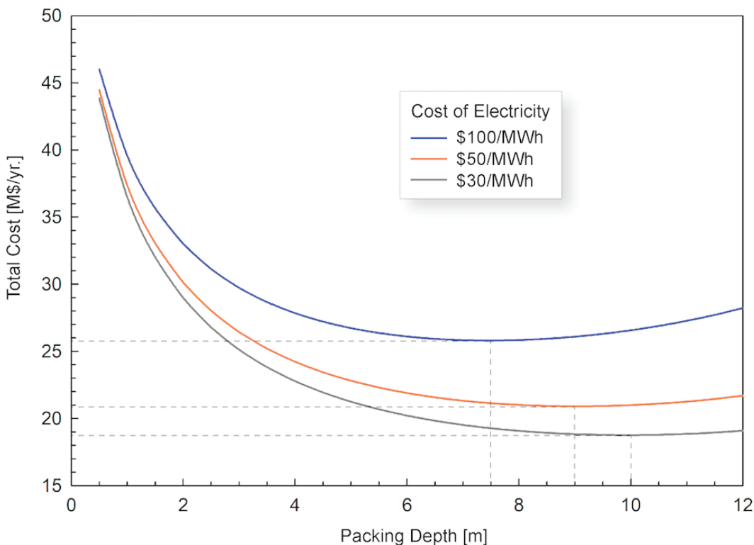
FIGURE 5.7 Relationship between packing depth and total cost of a direct air capture plant assuming costs of electricity of $30, $50, and $100/MWh.
