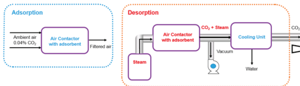
FIGURE 5.4 Schematic illustration of two-step, sorbent-based direct air capture process. NOTES: (1) Air contacts the sorbent using a gas-solid contactor (left) and (2) a heating system with possible application of vacuum is used to desorb the CO 2 from the sorbent followed by cooling before returning to the initial state (right).
