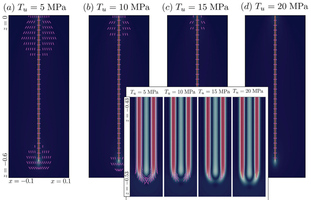
FIGURE 6.16 Pink lines indicate position and length of tensile fractures that would form in 2D model of a tabular zone of high porosity infiltrated by CO 2 -rich fluid, reacting with olivine to produce carbonate minerals with volume expansion. Panels labeled (a)-(d) illustrate results of a model without surface energy driven “capillary” flow, as a function of the tensile stress required for fracture, labeled at the top of each panel. The inset illustrates results of a model including surface energy driven fluid flow. SOURCE: Evans et al., 2018.
