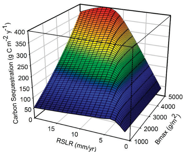
FIGURE 2.3 Carbon sequestration is a function of the rate of relative sea level rise (RSLR) and maximum marsh biomass ( B_{max} ) as depicted by simulations of the Marsh Equilibrium Model. SOURCE: James Morris, presentation to committee.
