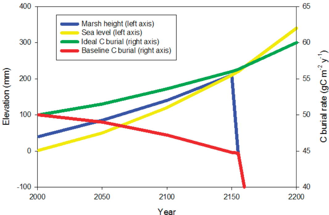
FIGURE 2.4 Hypothetical projection of marsh height (blue), sea level (yellow), ideal carbon burial rates (green), and baseline carbon burial rates without human intervention (red). NOTES: Impact of relative rate of SLR exceeds the growth in elevation of tidal wetlands until the year 2150 (in this example) when the marsh collapses. Without human intervention, the projected baseline of carbon burial rates decreases from the current 50 \text{ g}/(\text{m}^2 \text{ y}) \text{ C} to 0 in year 2150 when the marsh collapses.
