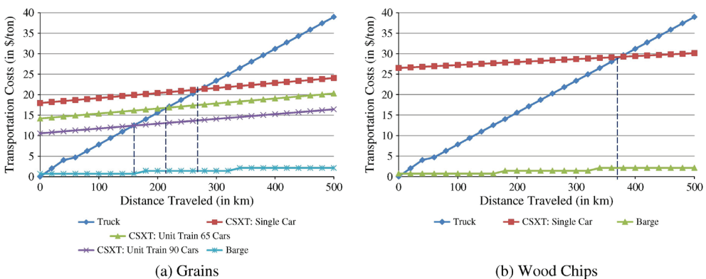
FIGURE 4.4 Transportation costs for (a) grains and (b) wood chips from Midwest to East and Southeast United States.
