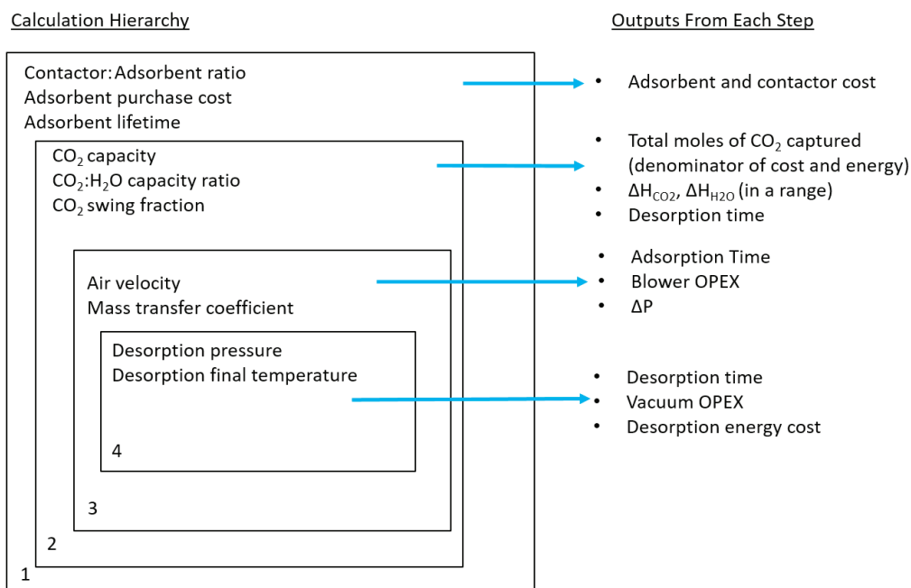
FIGURE D.2 Approach to calculating energy costs and process economics for a generic adsorption-based air capture process.
