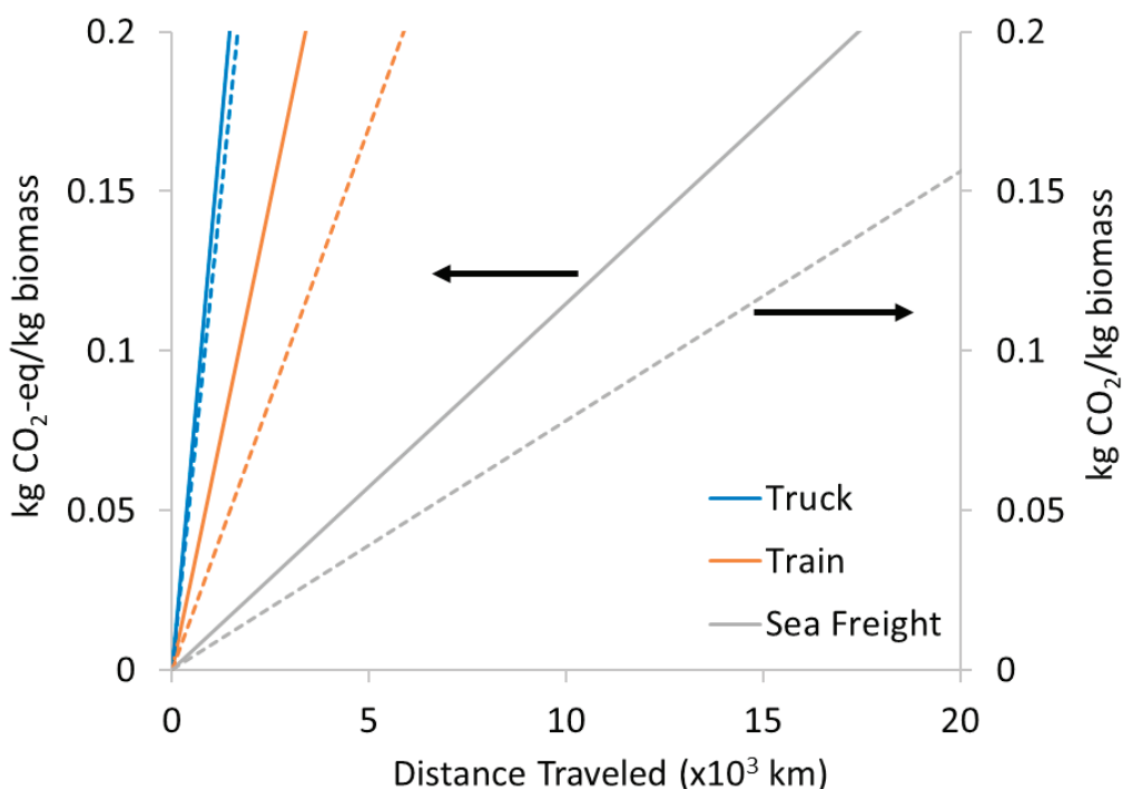
FIGURE 4.5 CO 2 and CO 2 e emissions per dry biomass produced as a function of transportation distance by road, rail, or sea.
