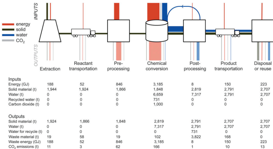
FIGURE E.1 Material and energy flows for an ex situ mineral carbonation process based on a carbonation rate of 1000 tCO 2 /day using and an olivine feedstock at 155 and 100 bar.
